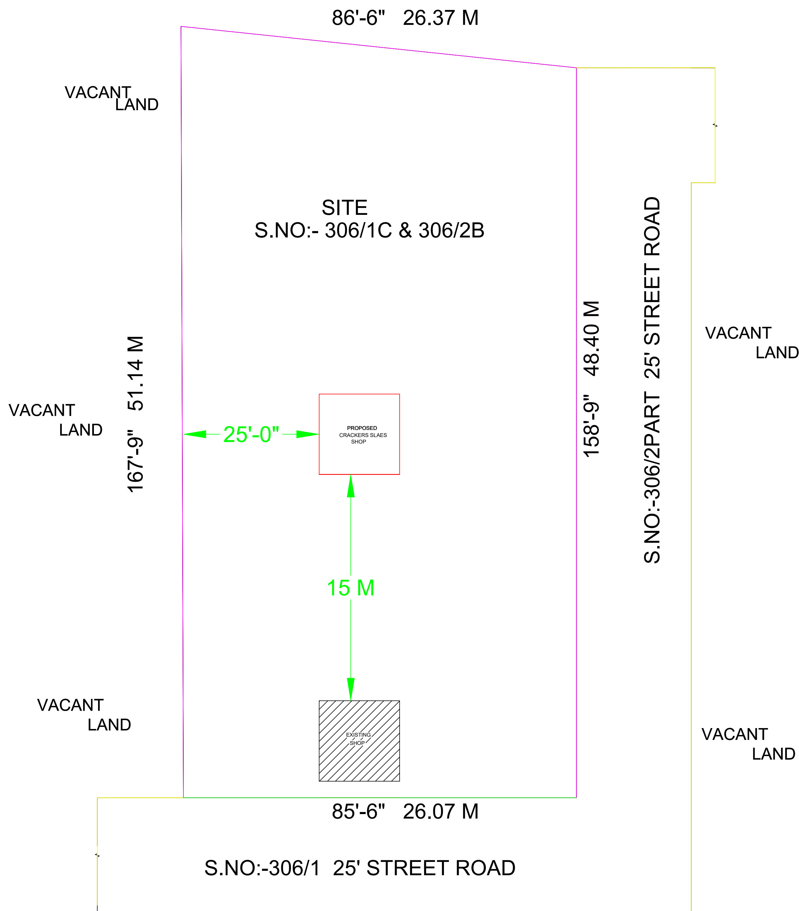
SITE PLAN
