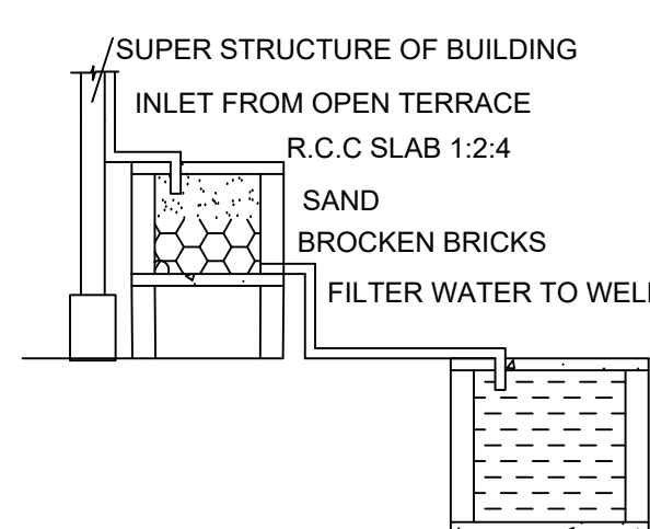
RAINWATER HARVESTING
