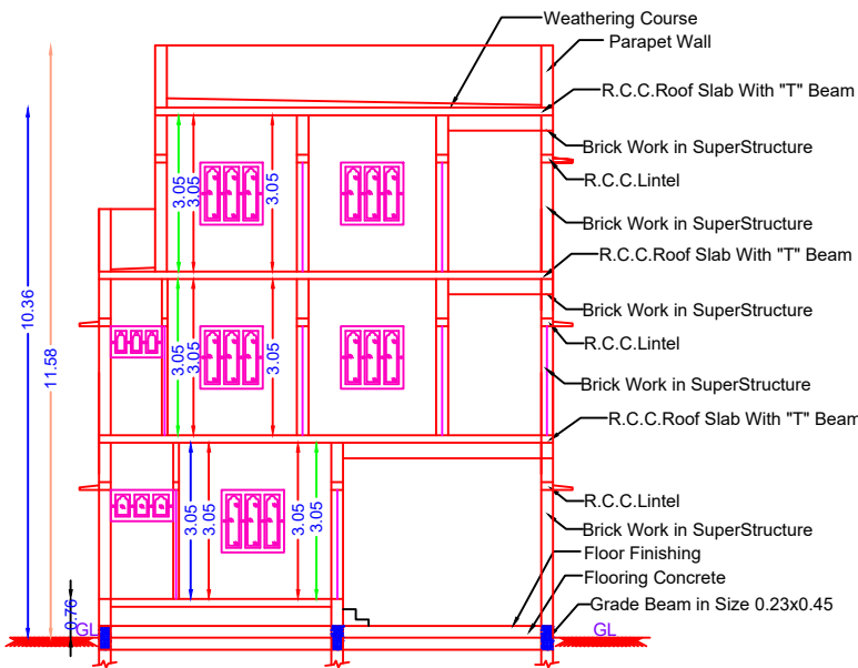
SECTION ON "PQ"
