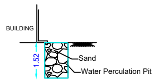
DETAILS OF RAIN WATER PERCOLATION PIT
