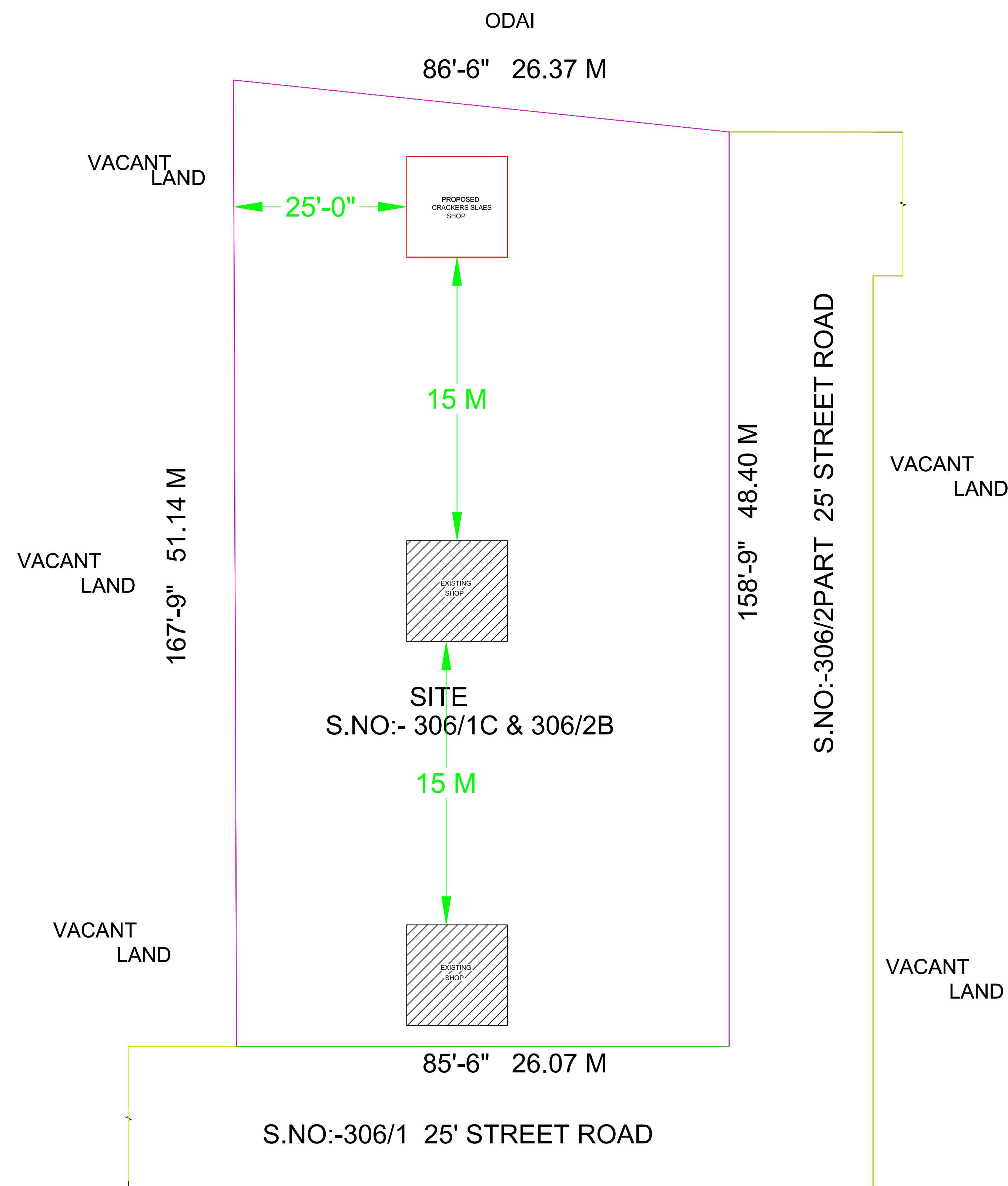
SITE PLAN
