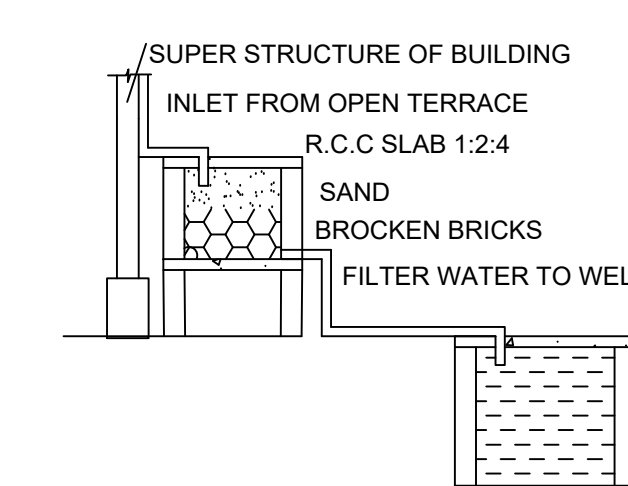
RAINWATER HARVESTING
