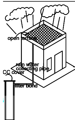
WH_CAPACITY_L=1000 RAIN WATER HARVESTING ARRANGEMENT
