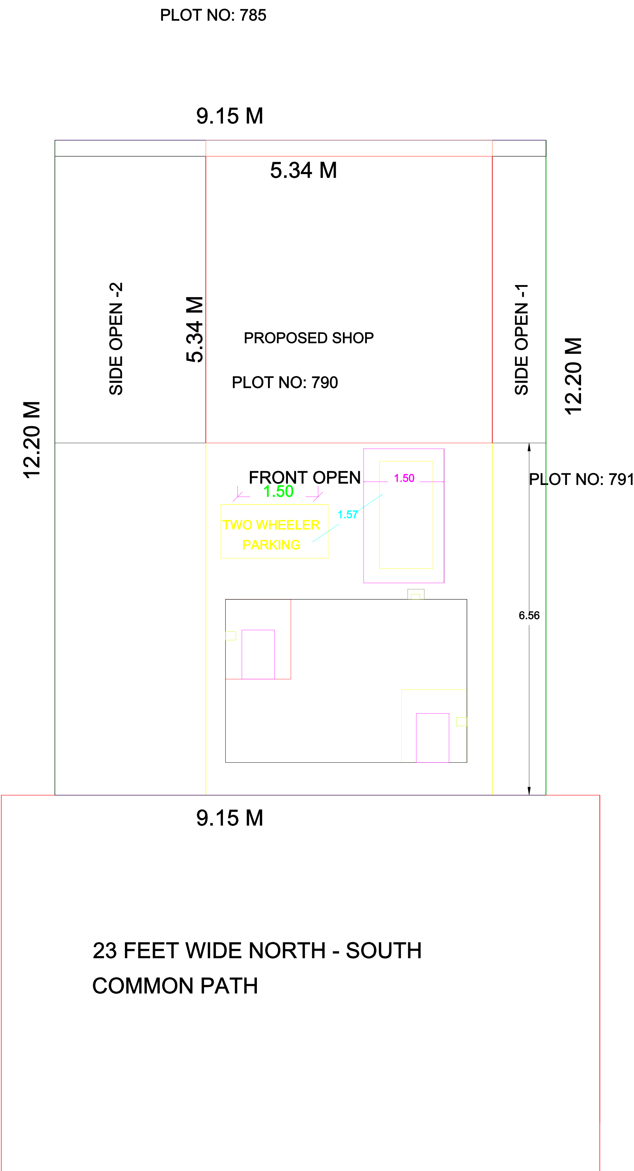
SITE PLAN
