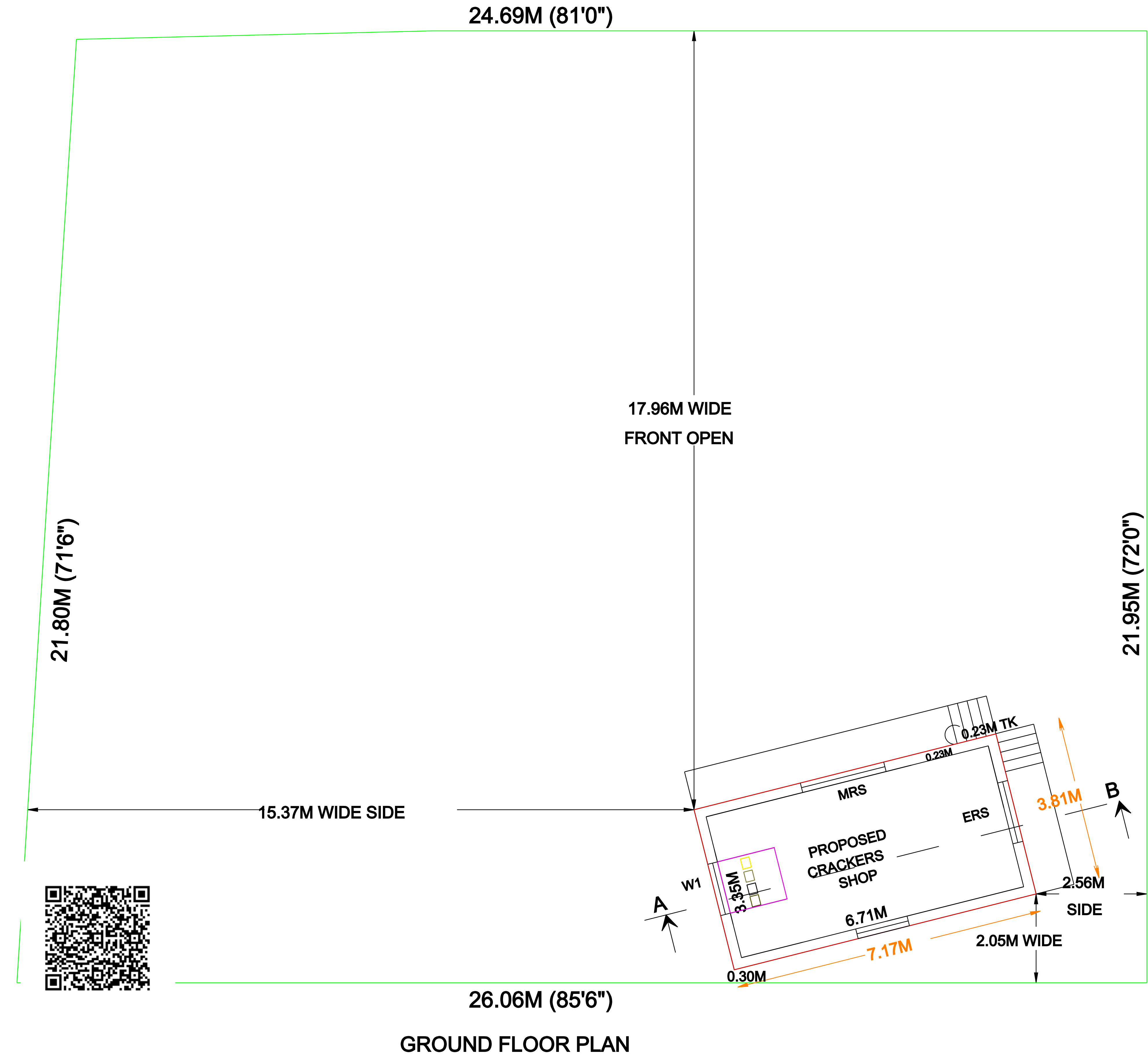
LOCATION PLAN
