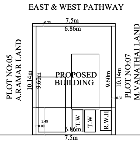
12' WIDE EAST & WEST STREET
