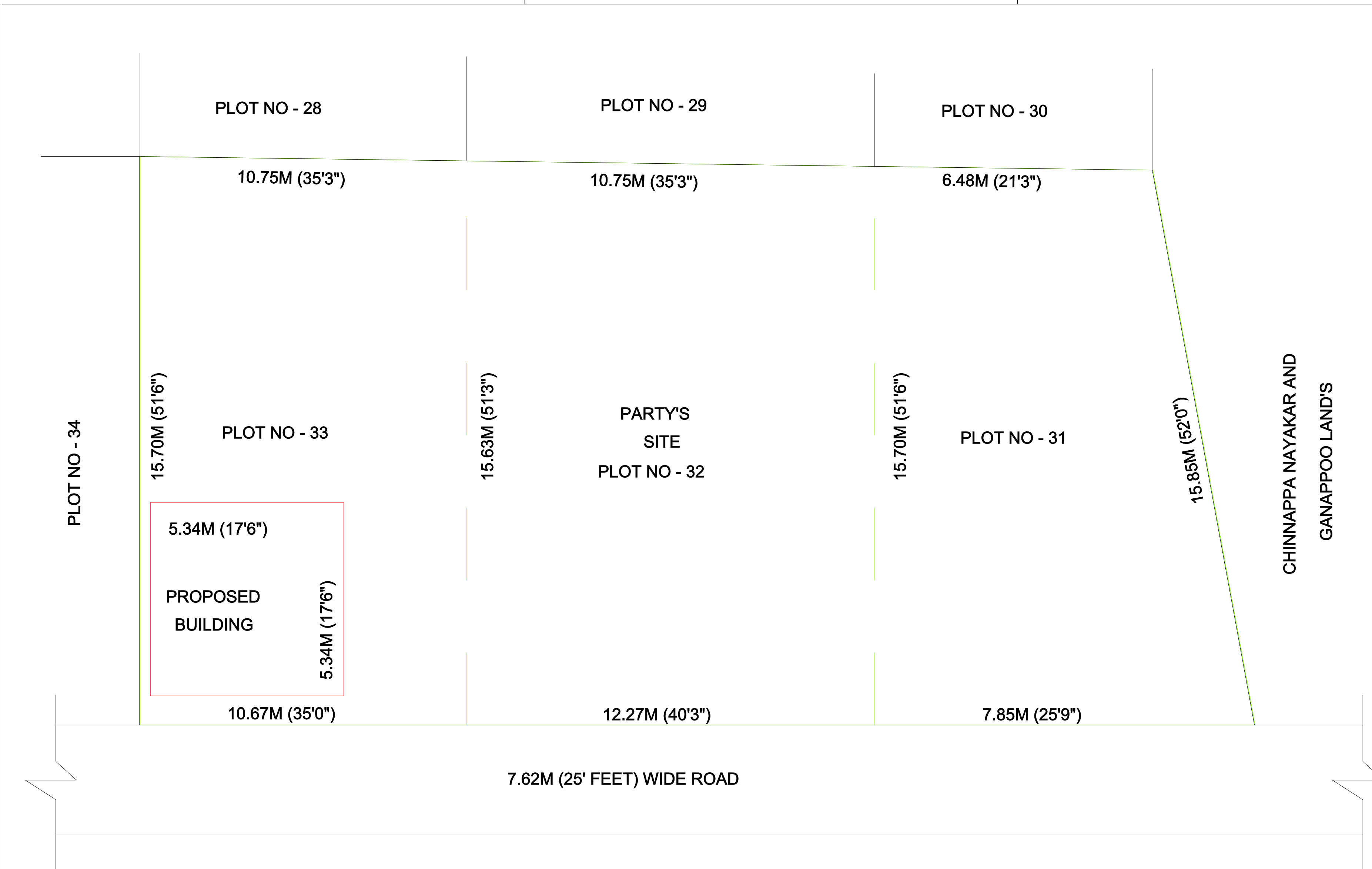
SITE PLAN
