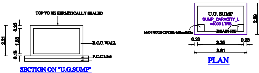
SECTION ON "U.G.SUMP"
