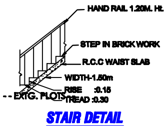
STAIR DETAIL
