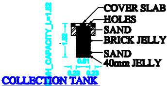
SECTION OF RAIN WATER
