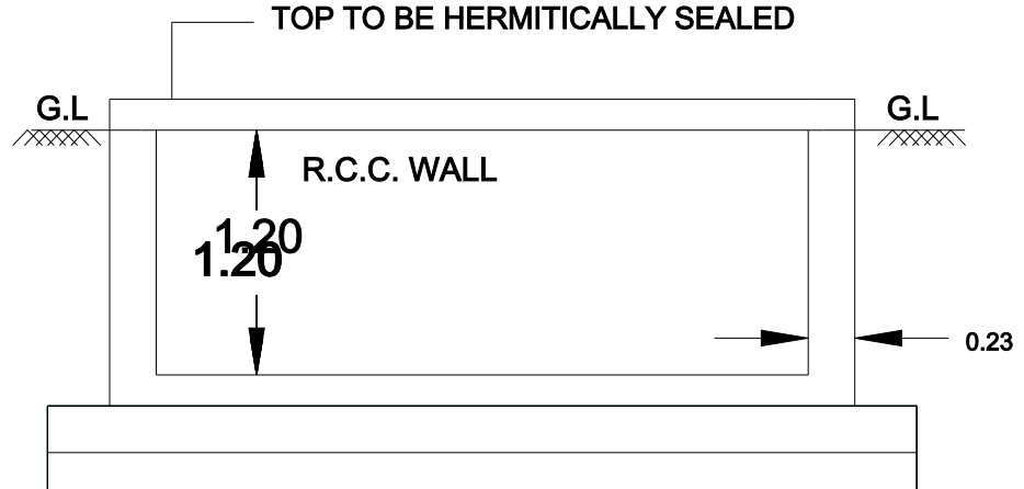
RWH_CAPACITY_L = 2000
