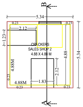
GROUND FLOOR PLAN-2
