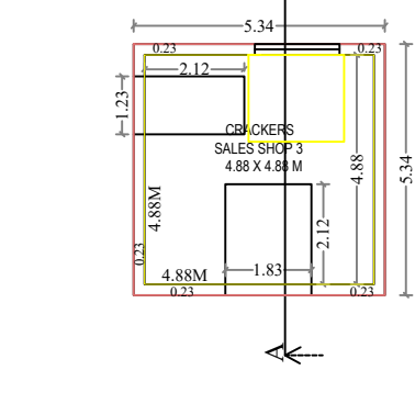
GROUND FLOOR PLAN-4
