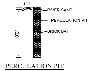
PERCOLATION PIT
