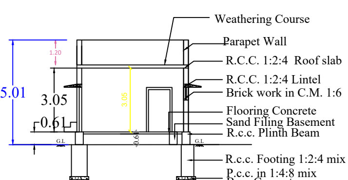
SECTION -"AB"
