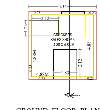
GROUND FLOOR PLAN-5
