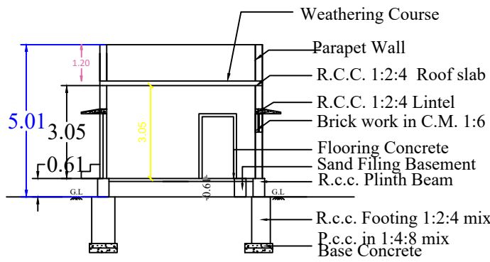
SECTION -"AB"
