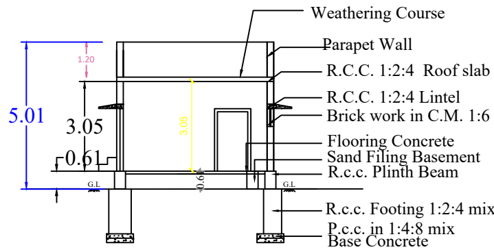
SECTION -"AB"
