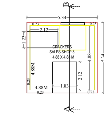
GROUND FLOOR PLAN-1
