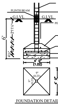
FOUNDATION DETAIL
