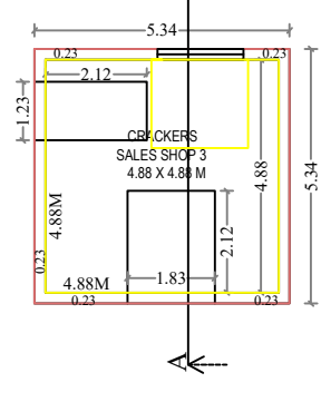
GROUND FLOOR PLAN-3
