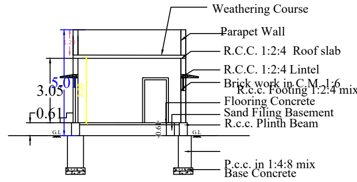
SECTION -"AB"
