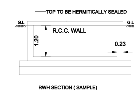
RCC SECTION (SAMPLE)
