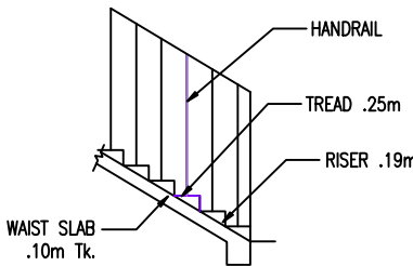
STAIR DETAIL
