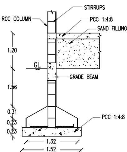
COLUMN DETAILS
