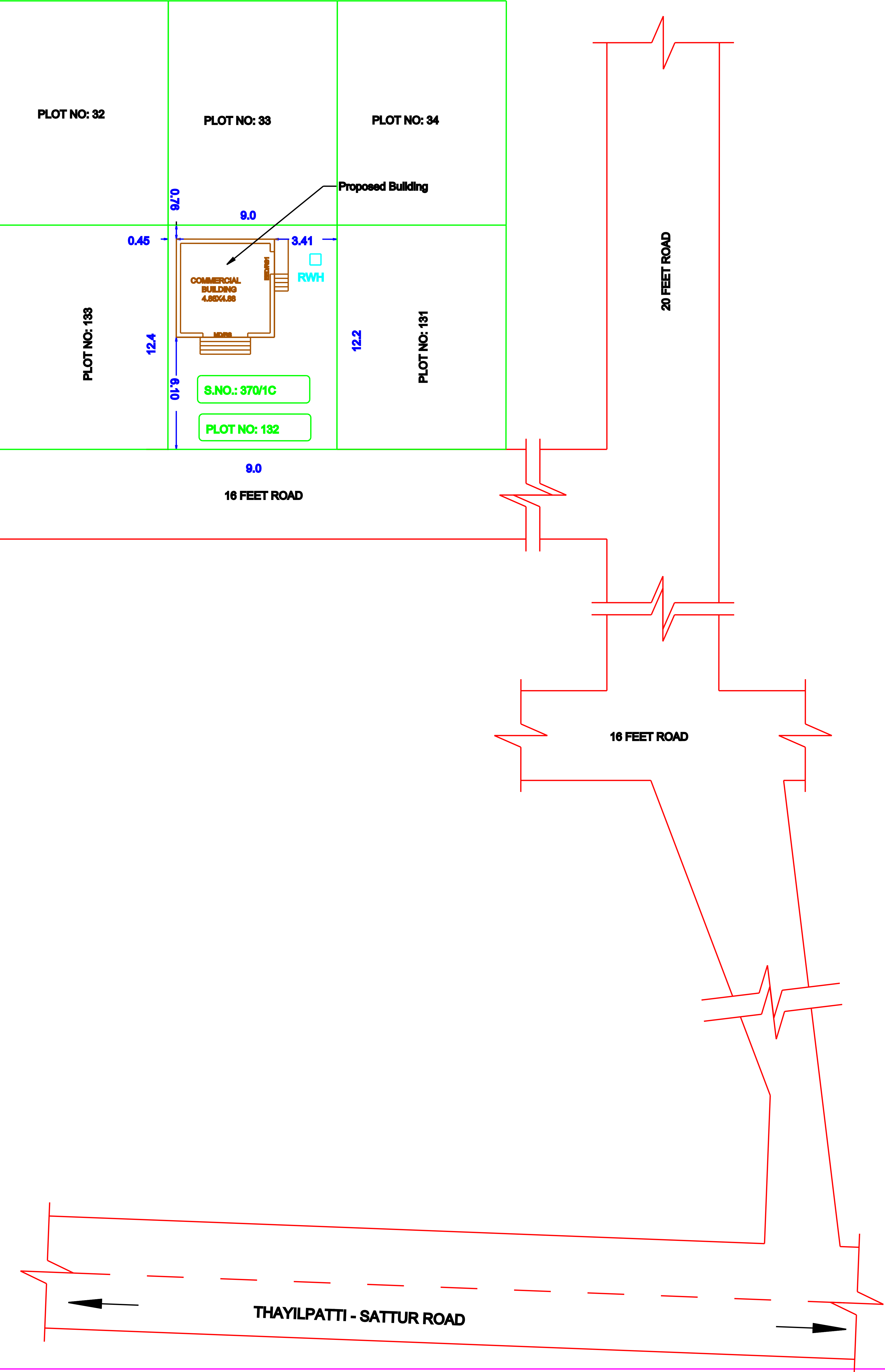
SITE PLAN SCALE 1:200
