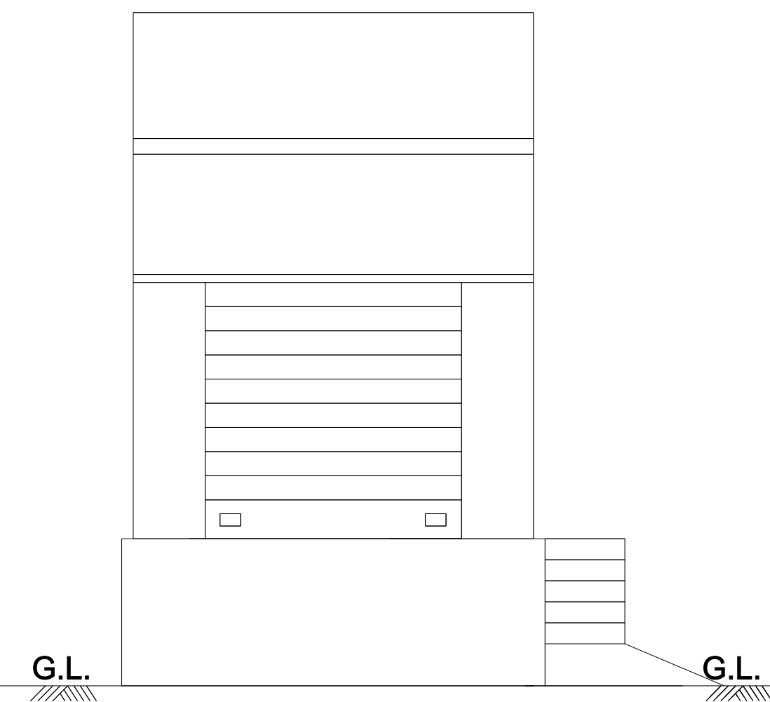
FRONT ELEVATION
