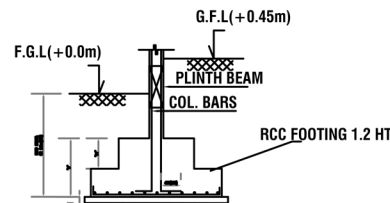
SECTION X-X OF FOOTING
