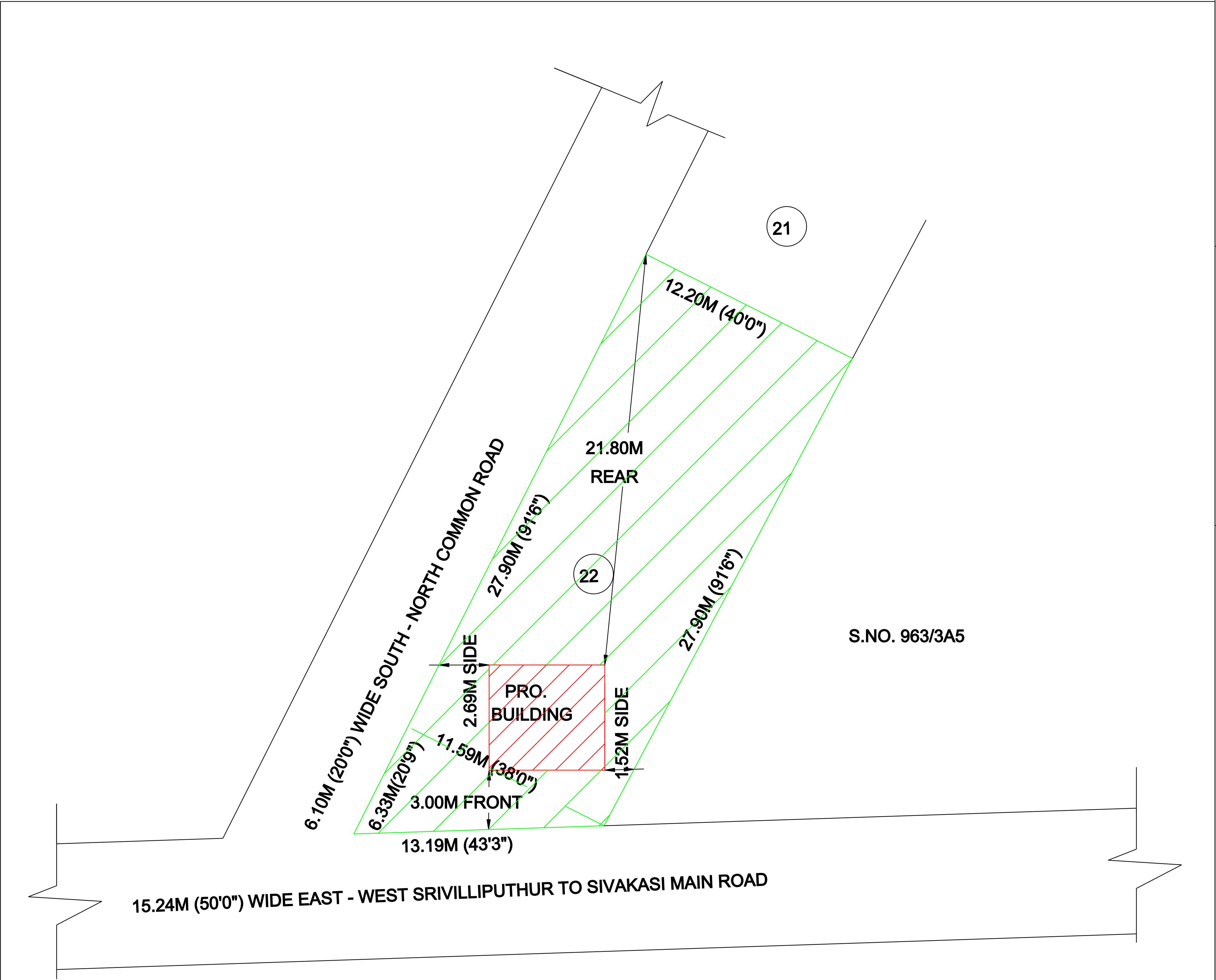
LOCATION PLAN
