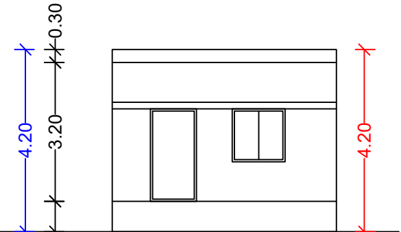
Front Elevation
