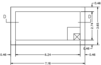
SCALE 1"=2'0"
