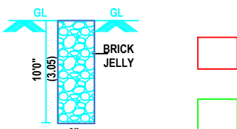
PERCULATION PIT
