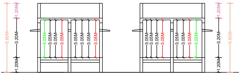
SECTION
