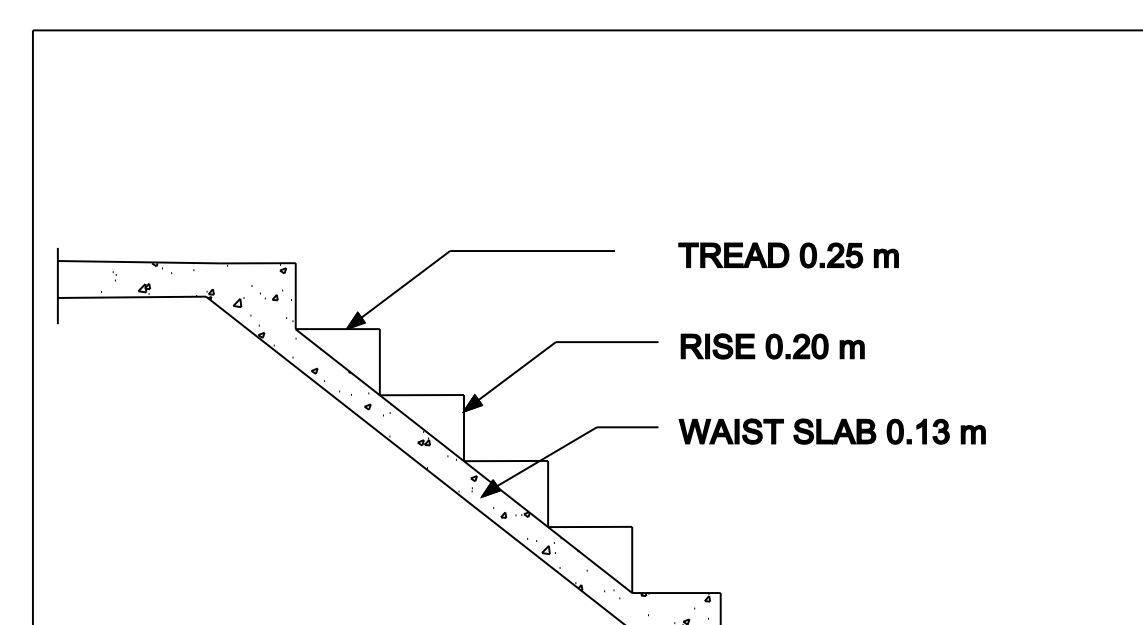
STAIR DETAILS
