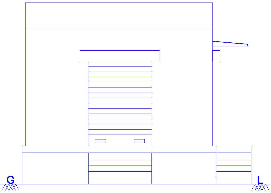
ELEVATION ON EAST SIDE
