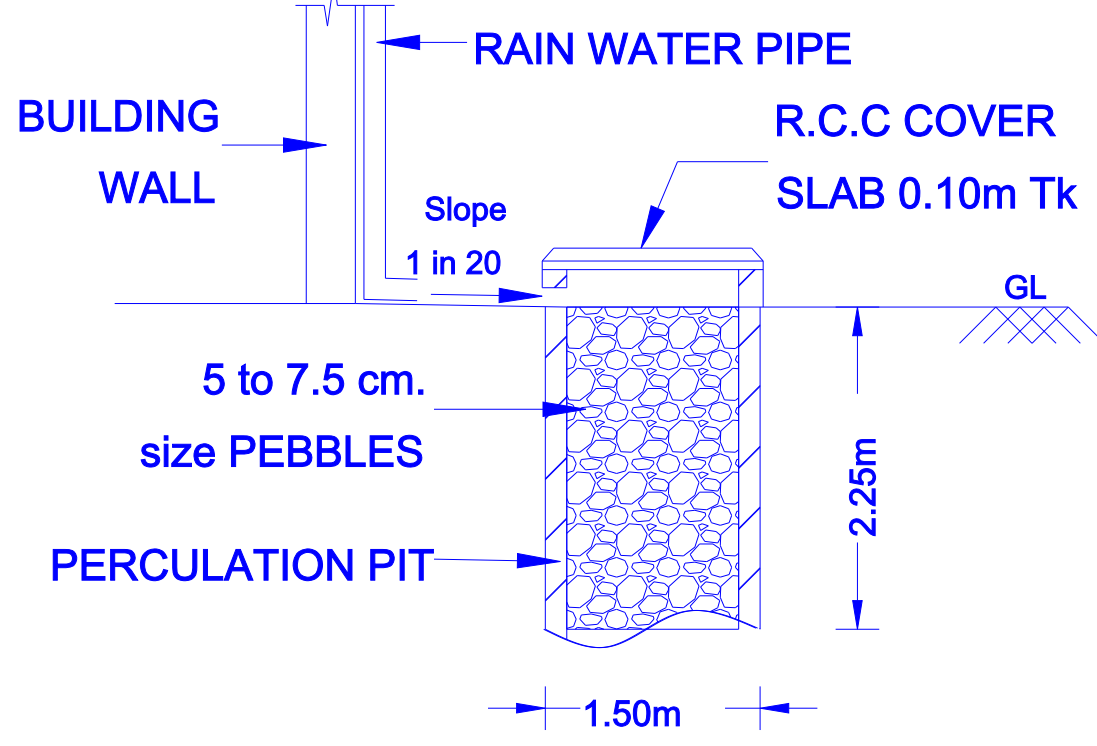
RAIN WATER HARVESTING TRENCH PIT DETAILS
