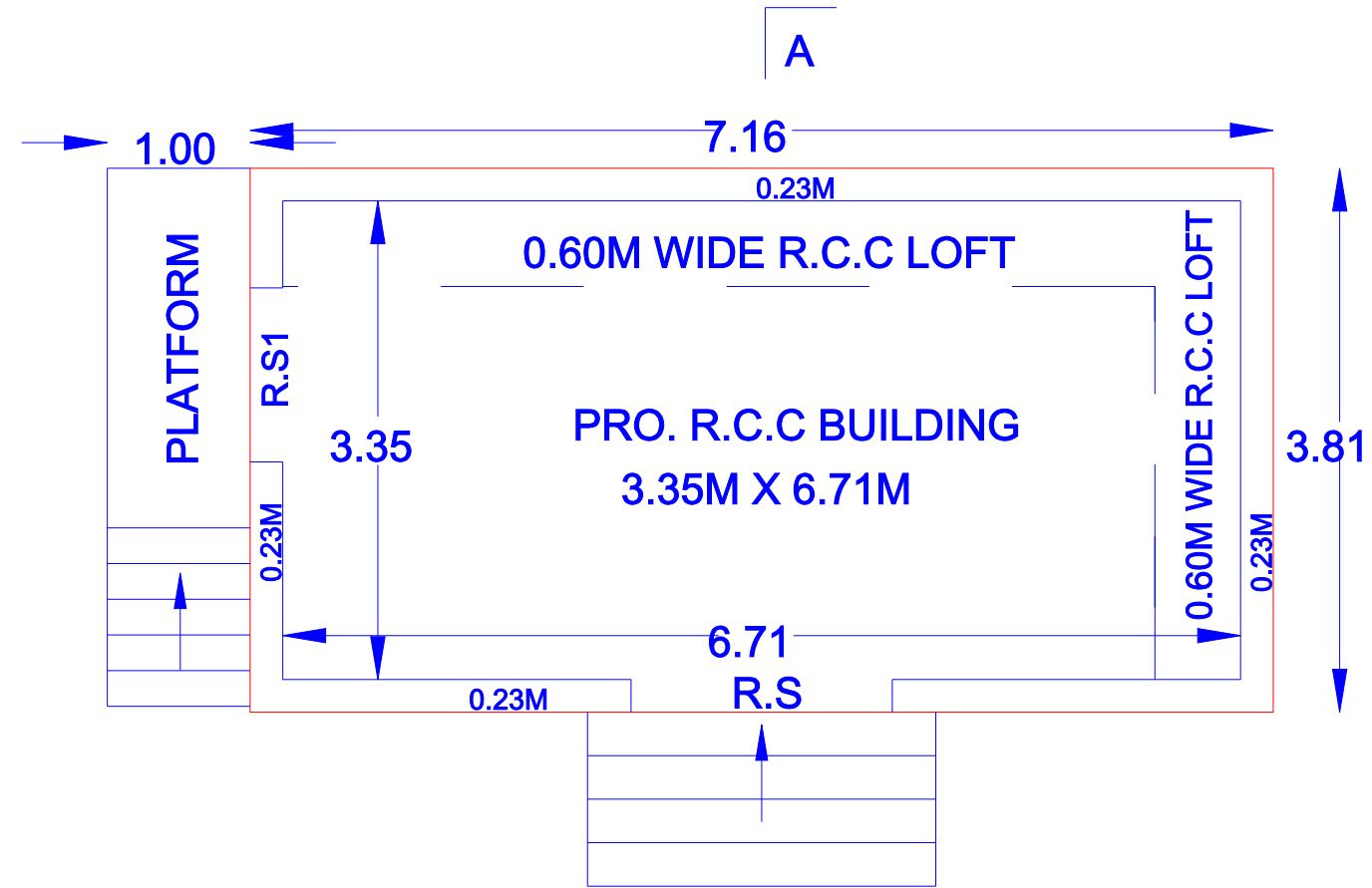
PRO. GROUND FLOOR PLAN
