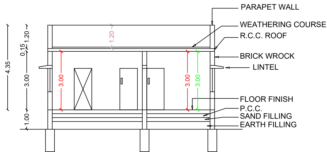
SECTION ON "XY"
