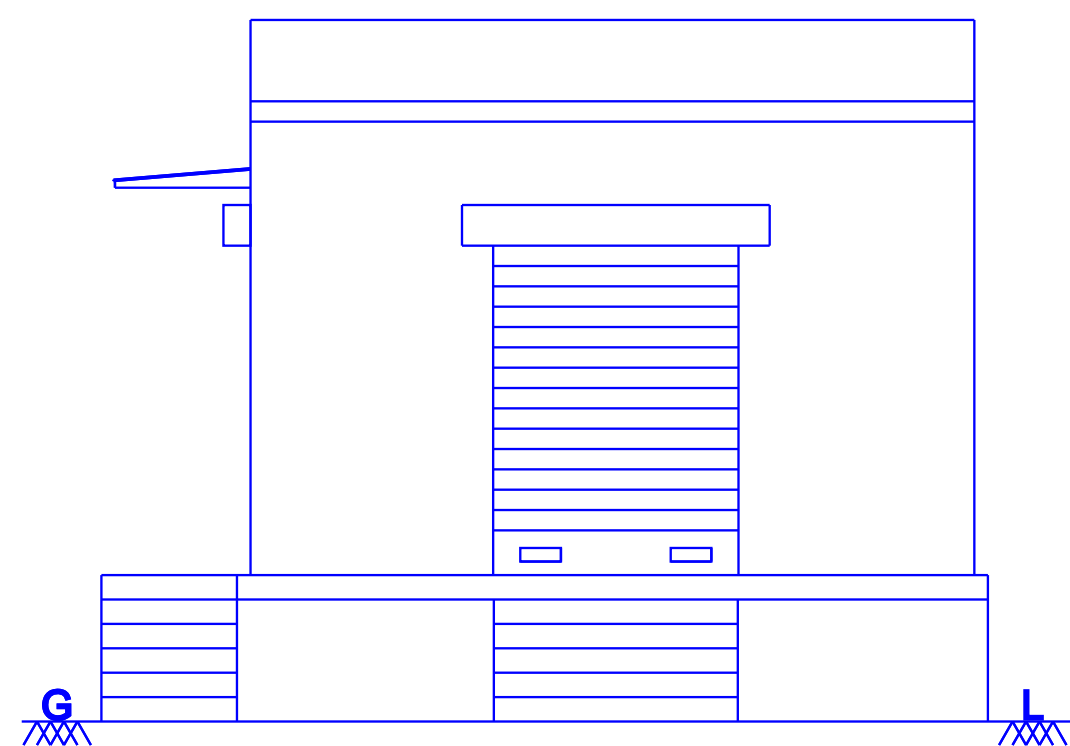
ELEVATION ON SOUTH SIDE
