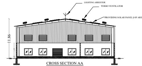
CROSS SECTION AA
