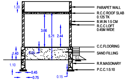
SECTION ON-AB
