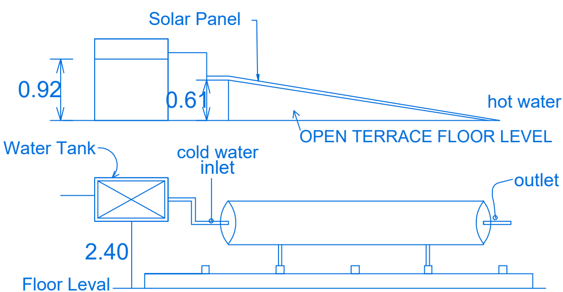
Details of solar water heating system
