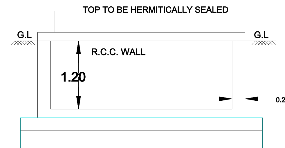
RWH_CAPACITY_L = 2000
