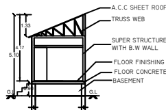
SECTION ON AA'
