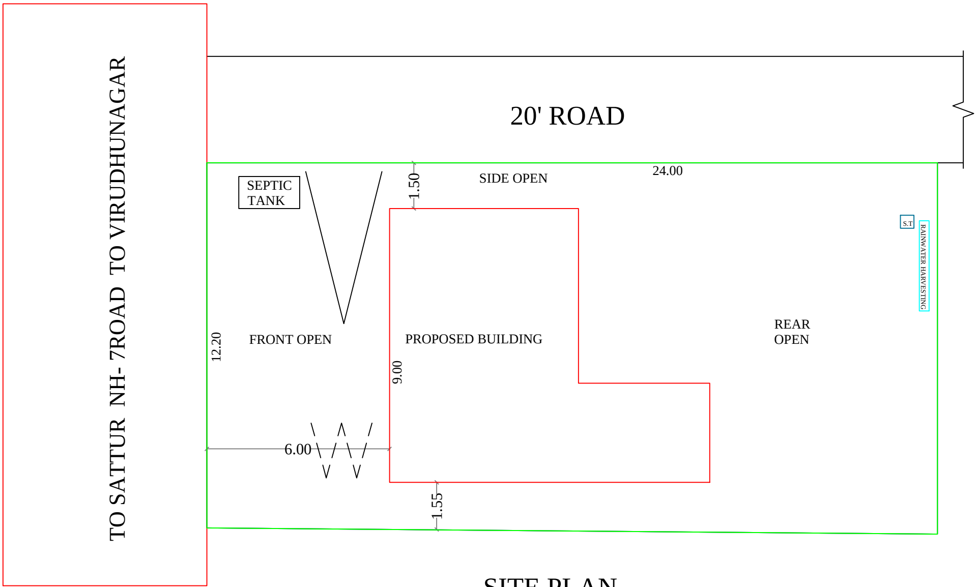
SITE PLAN
