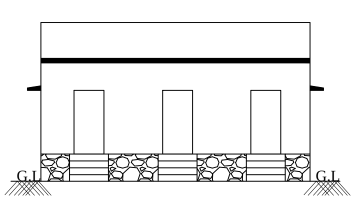
FRONT ELEVATION (WEST FACING)
