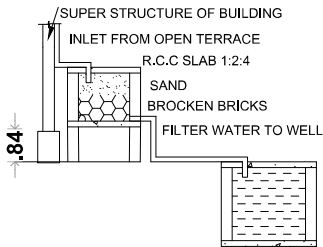
RAINWATER HARVESTING
