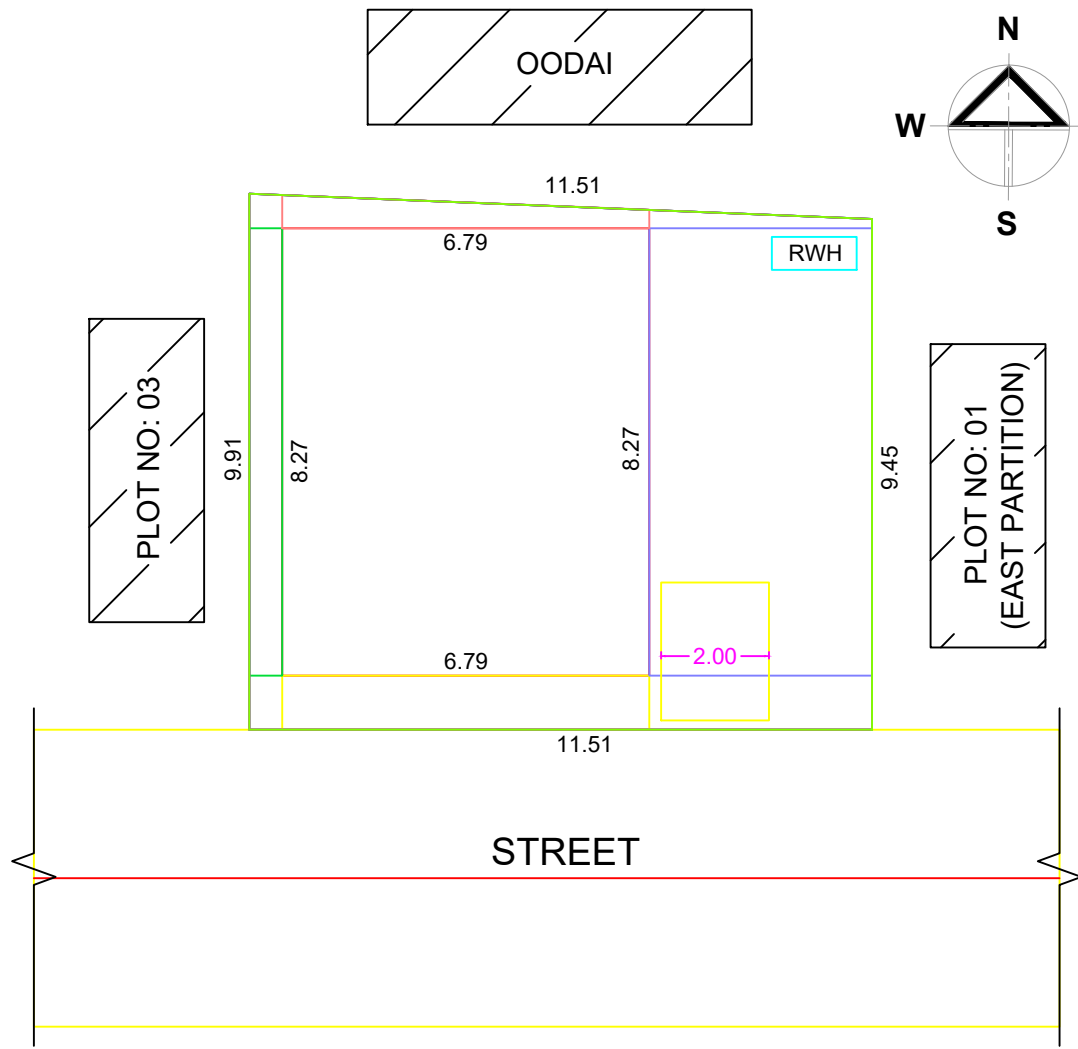
TOPO PLAN Scale 1:100
