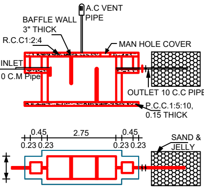
SEPTIC TANK AND TRECH
