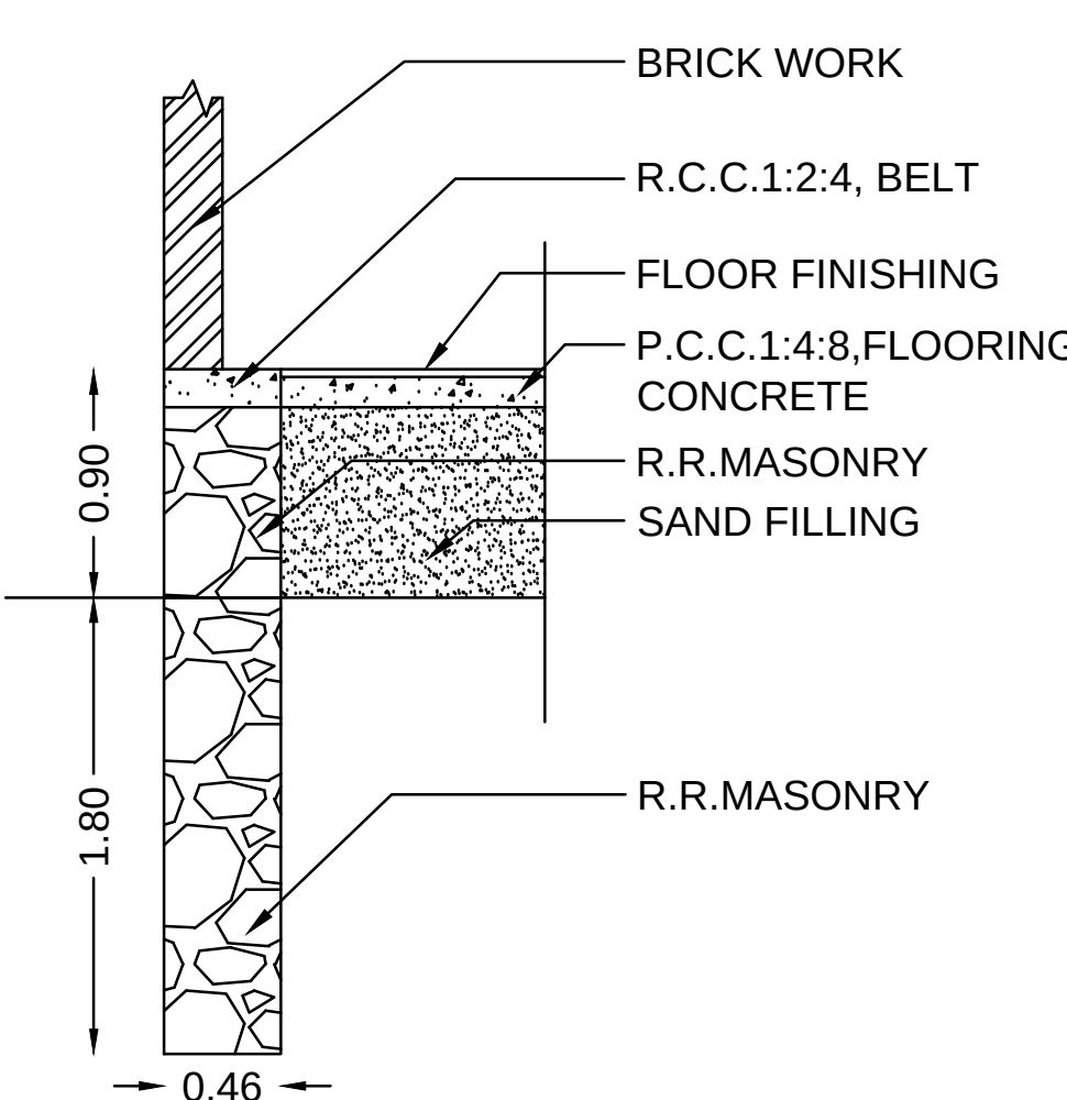
FOUNDATION DETAILS
