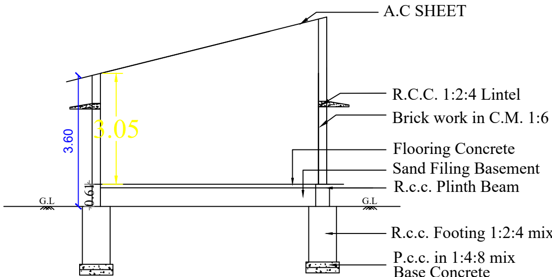
SECTION -"AB"
