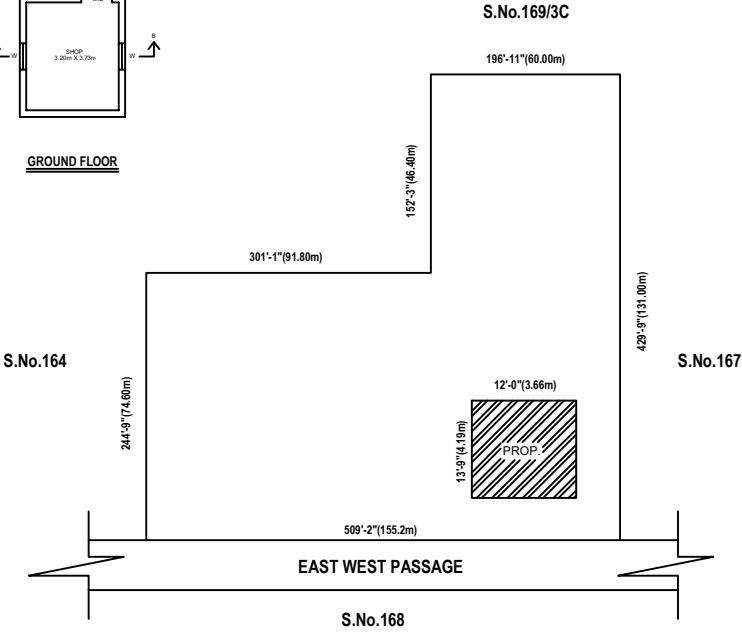
SITE PLAN
