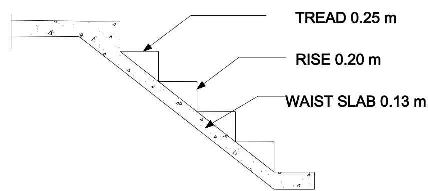
STAIR DETAILS
