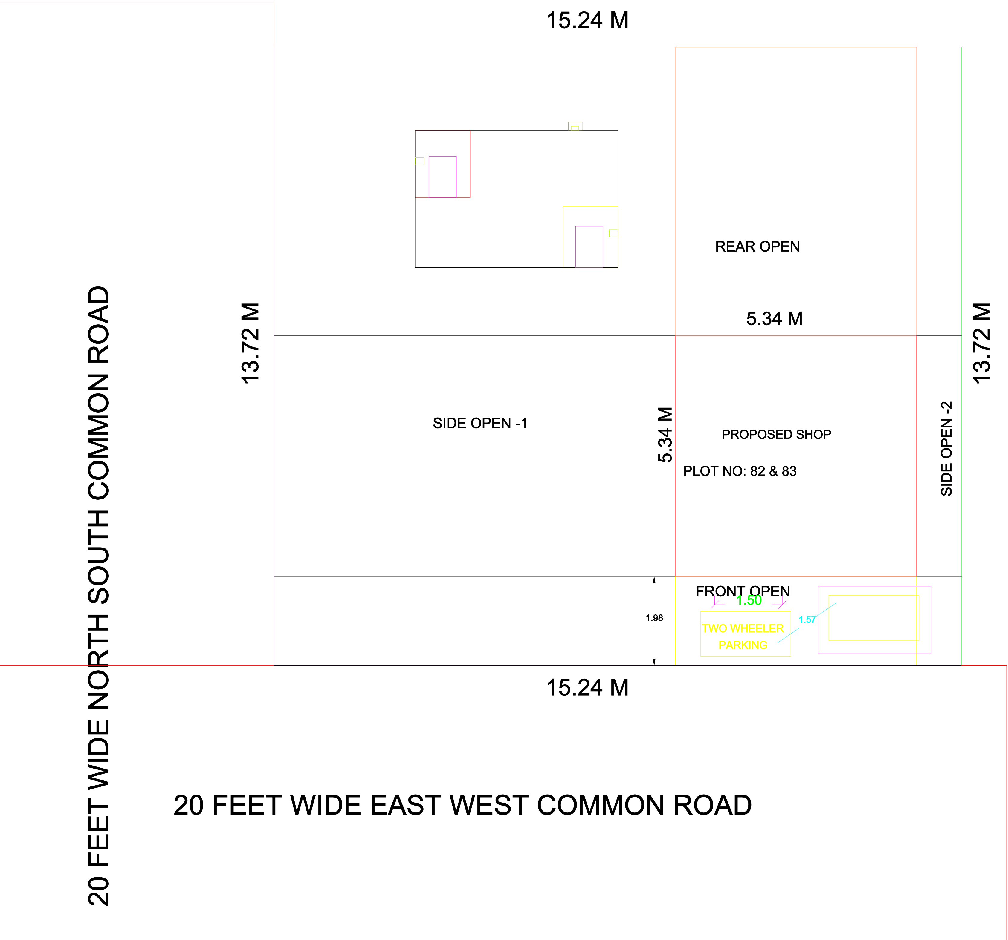
SITE PLAN
