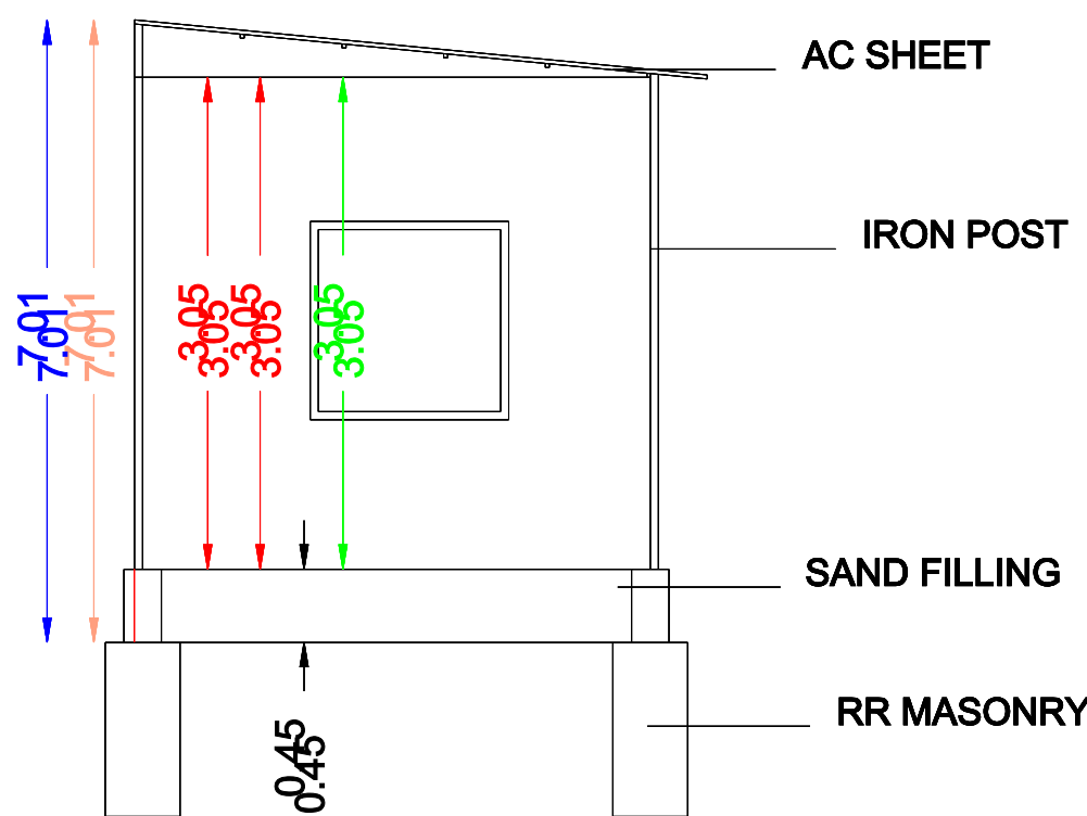
SECTION ON AC
