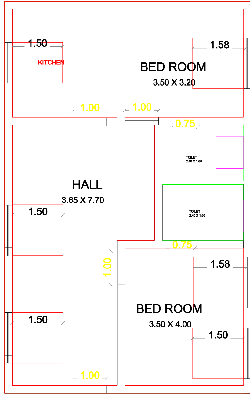
PLAN
