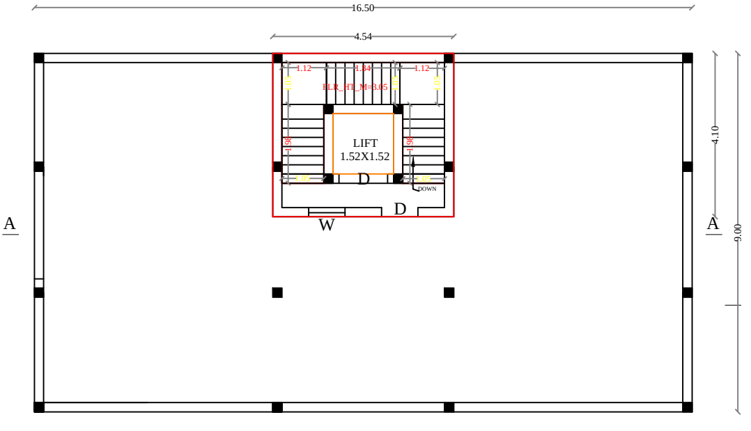
TERRACE FLOOR PLAN(TF)
