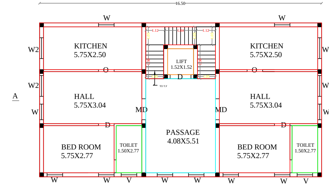
SECOND FLOOR PLAN(S.F)
