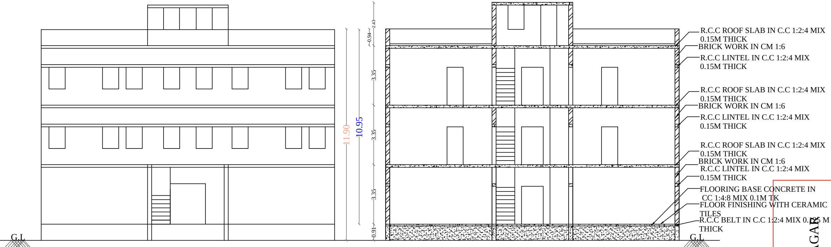
FRONT ELEVATION (FACING NORTH)
