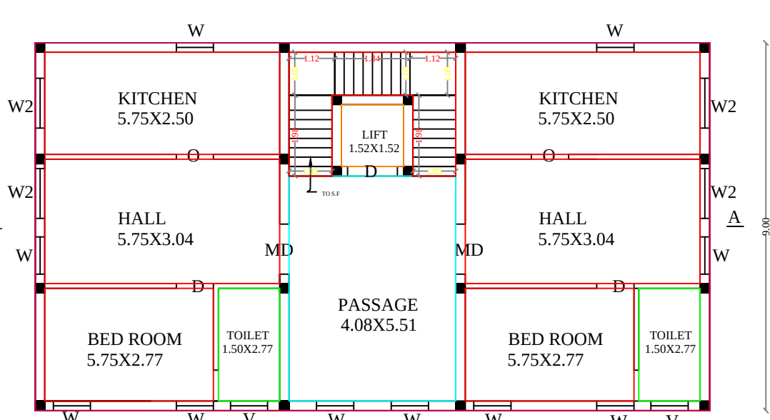
FIRST FLOOR PLAN(F.F)
