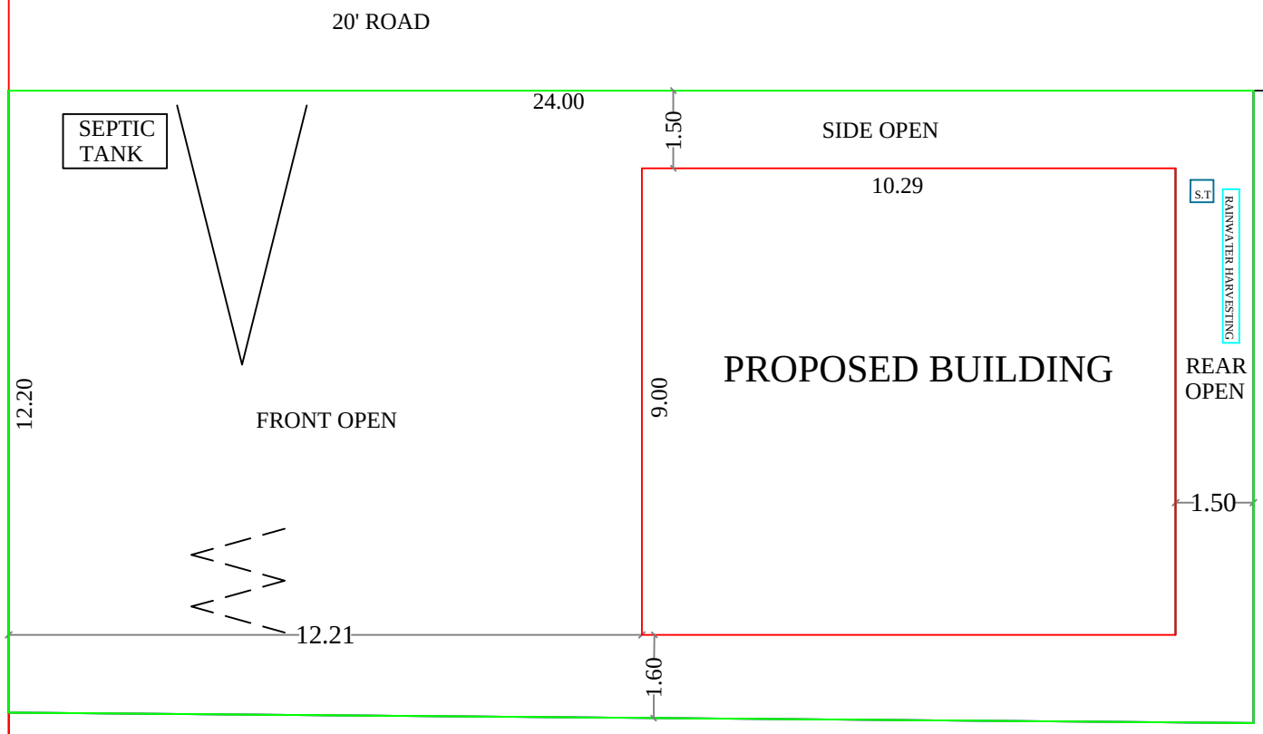
SITE PLAN
