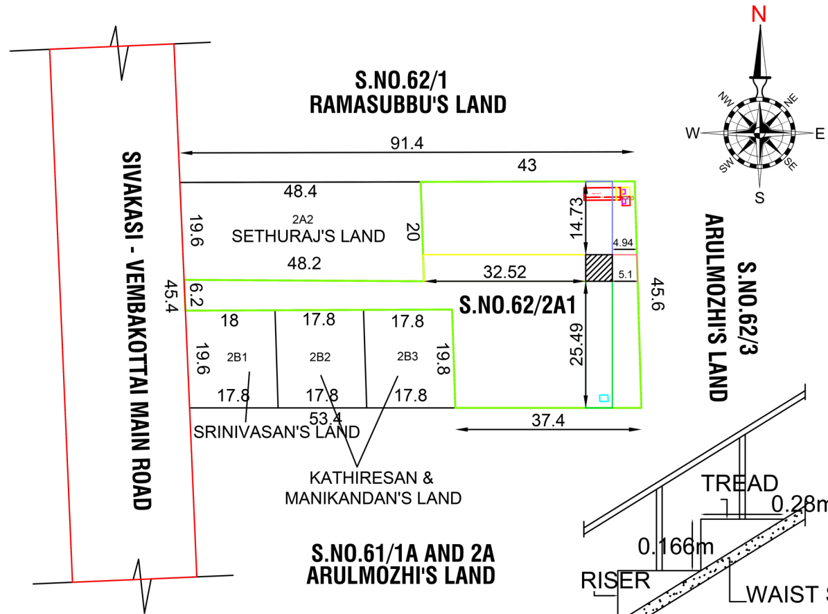
SITE CUM PLAN SCALE 1:100
