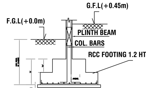
SECTION X-X OF FOOTING SCALE - 1:75
