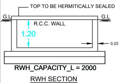
RWH SECTION
