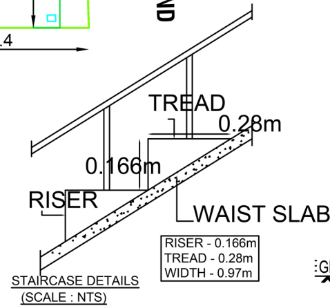
STAIRCASE DETAIL
