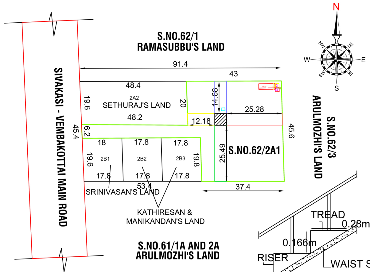
SITE CUM PLAN SCALE 1:100
