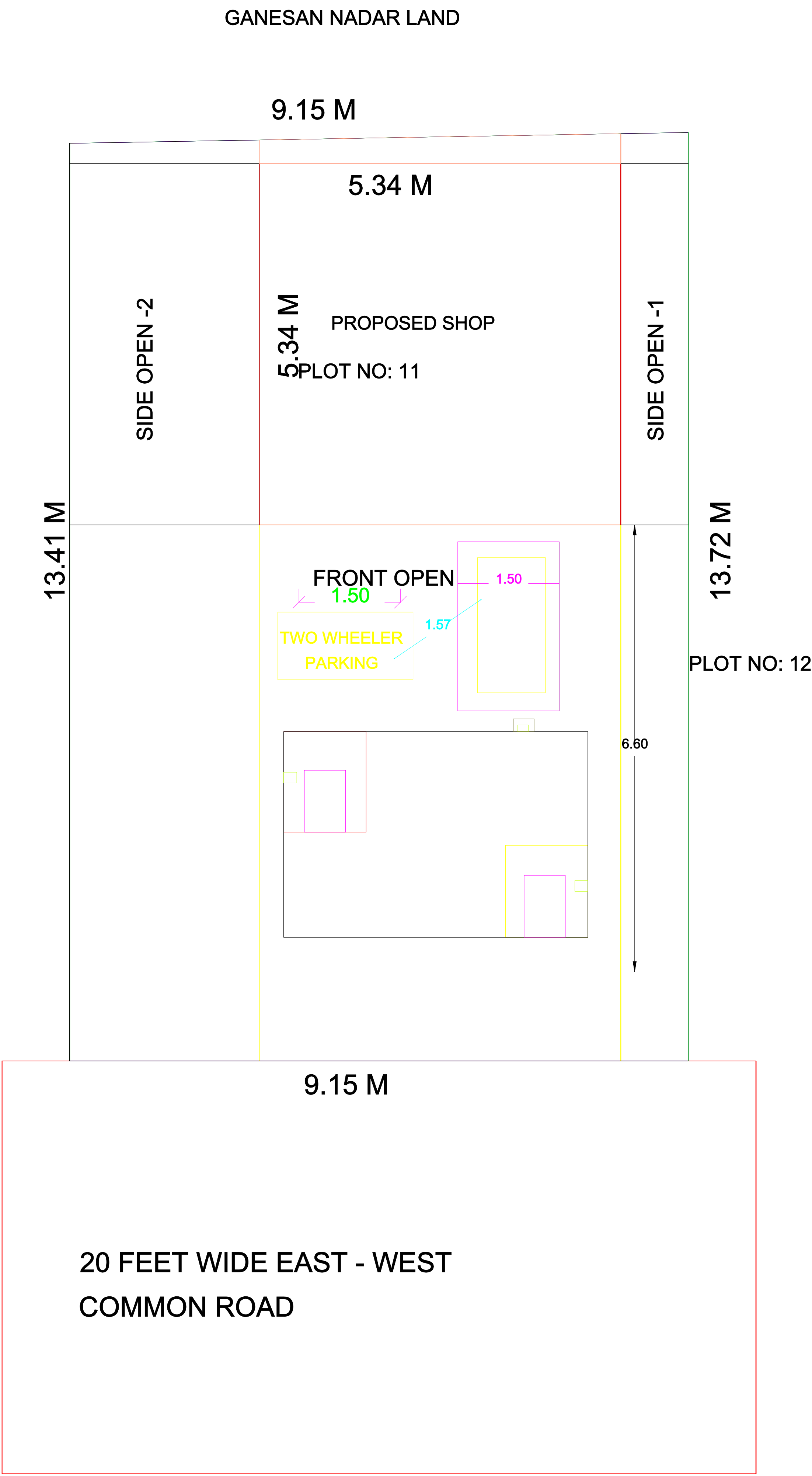
SITE PLAN
