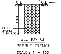
SECTION OF PEBBLE TRENCH SCALE : 1" = 100
