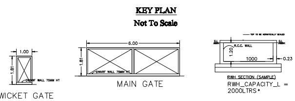
WICKET GATE
