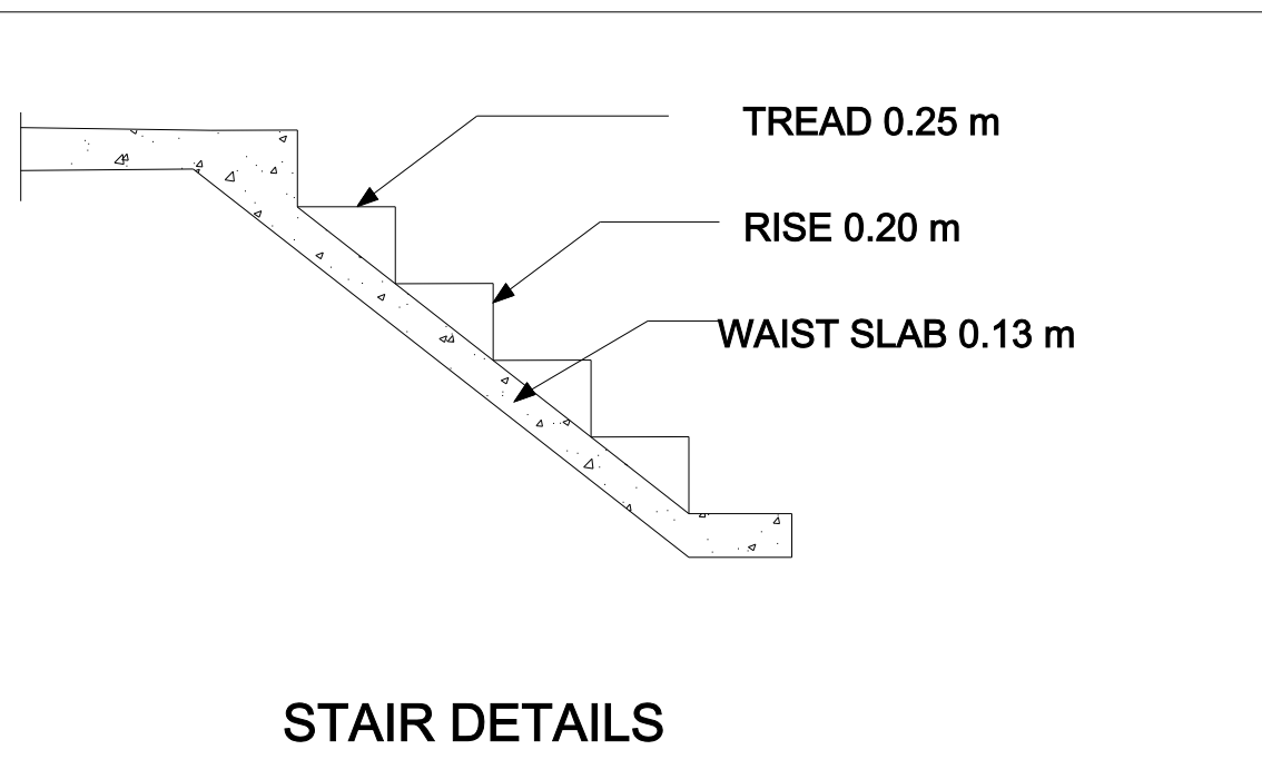
STAIR DETAILS
