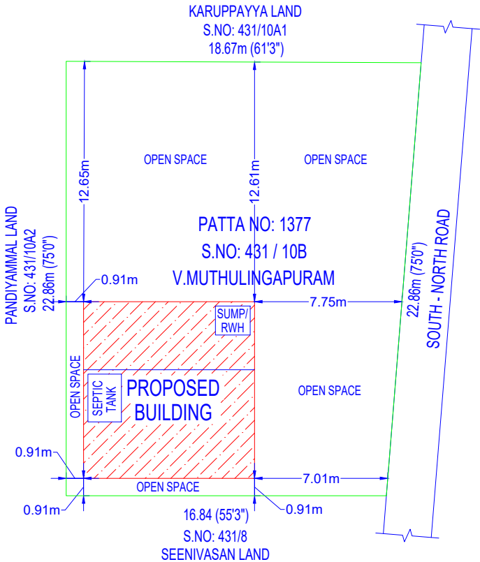
SITE PLAN
