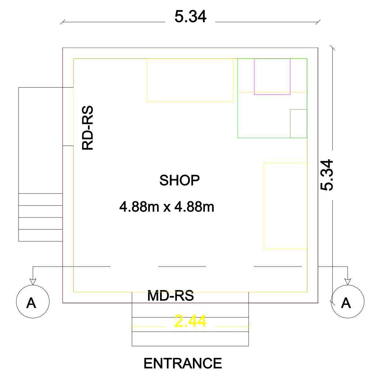
FLOOR PLAN
